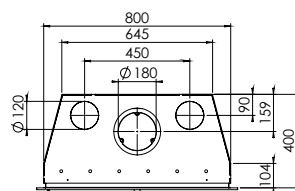
Instyle + Classic Line frame
