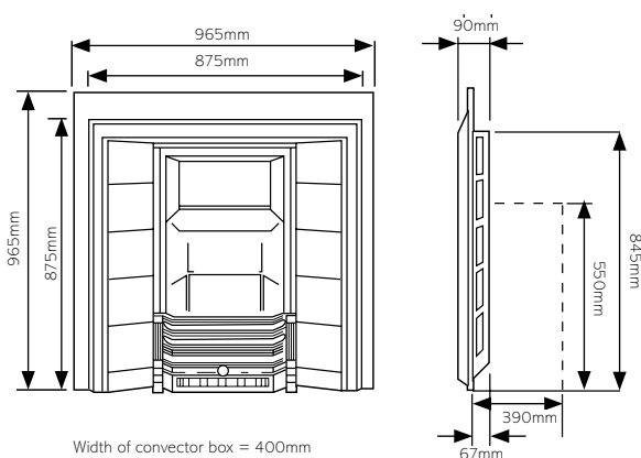
Victorian Tiled Convector
